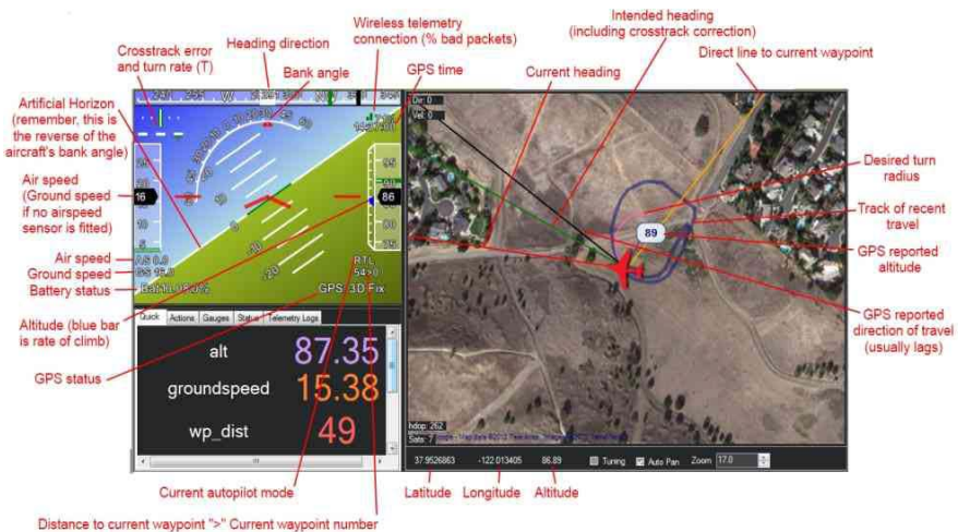
Figure 2-9. A Modern Autopilot Control, an Ardupilot Ground Control Station. 15
